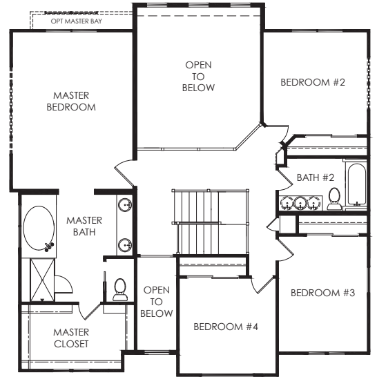
UPPER LEVEL 1,373 SF
