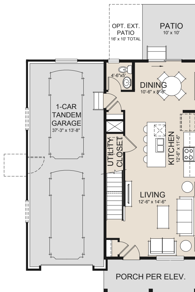
MAIN LEVEL 612 SF
