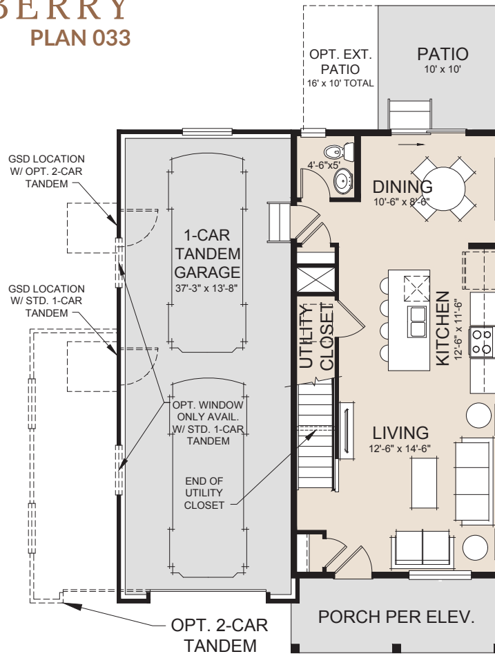
MAIN LEVEL 612 SF
