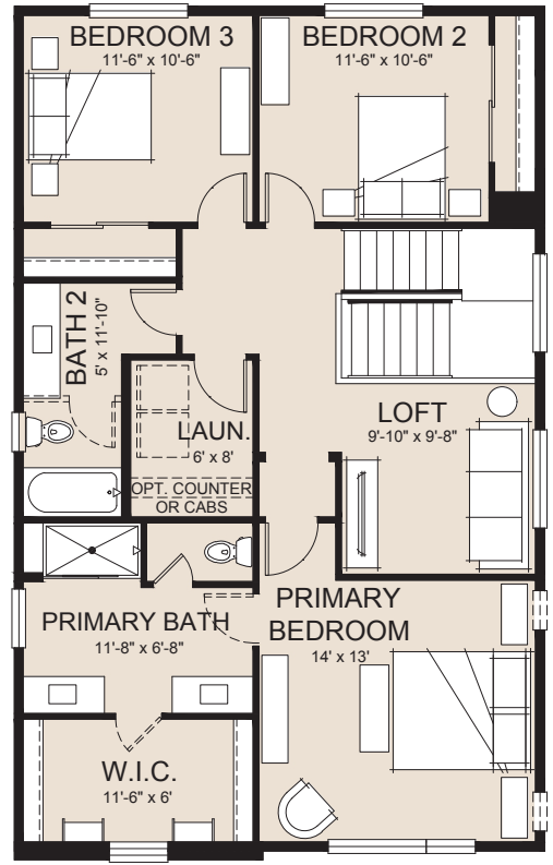
UPPER LEVEL 1,161 SF
