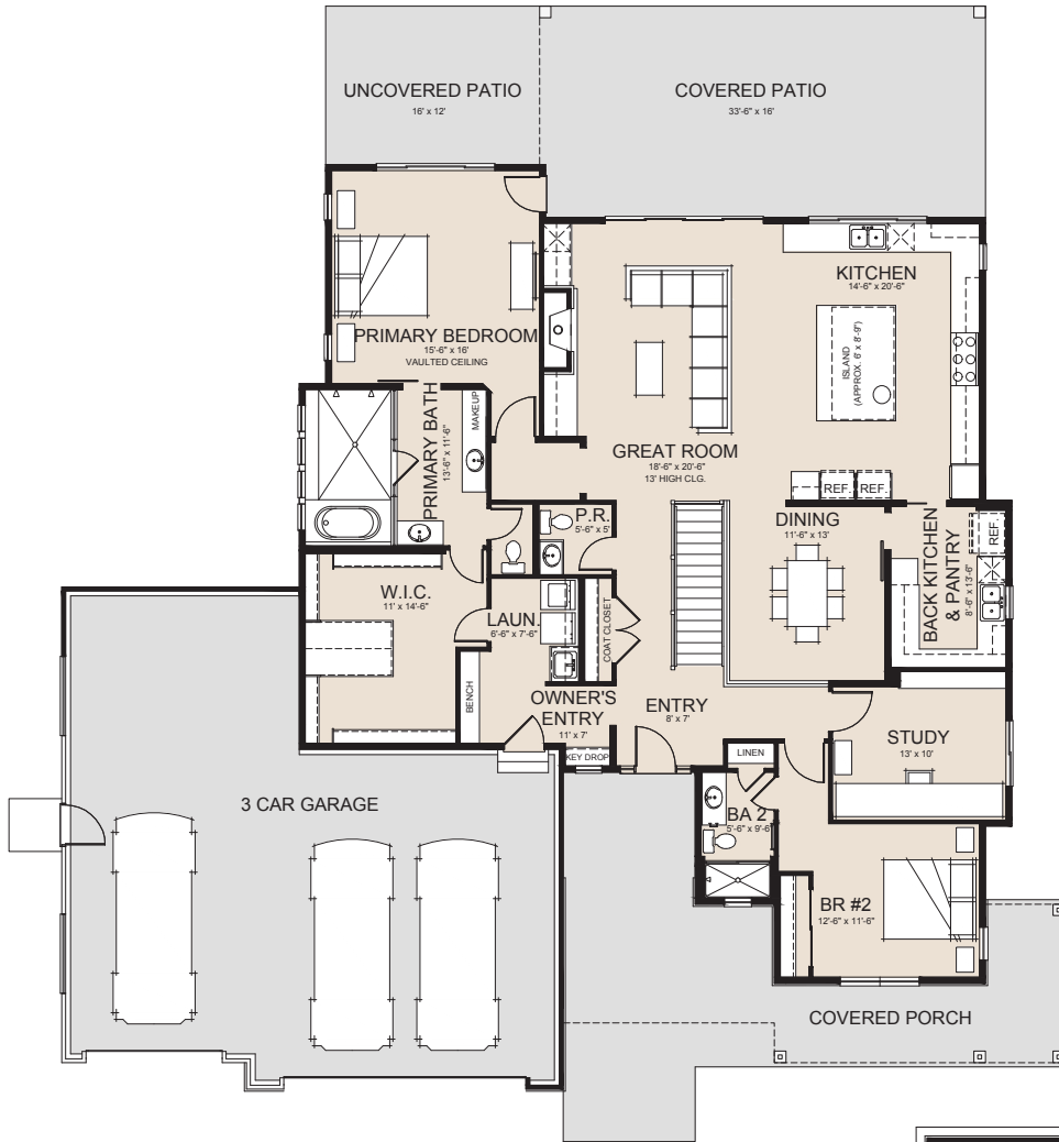
MAIN LEVEL 2,565 SF
