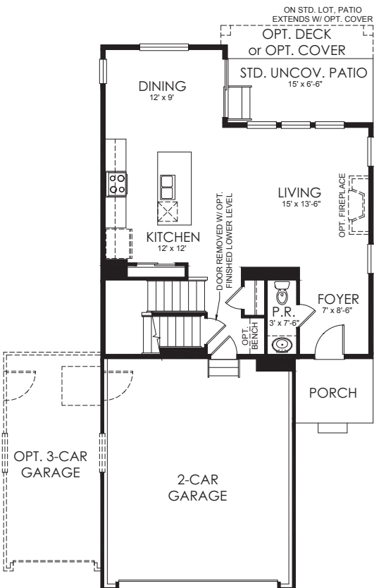
MAIN LEVEL 782 SF
