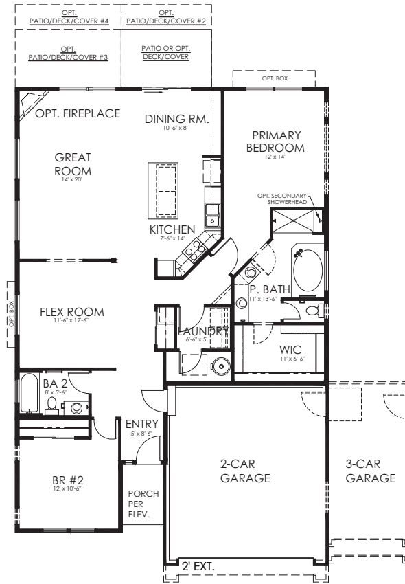
MAIN LEVEL 1,659 SF
