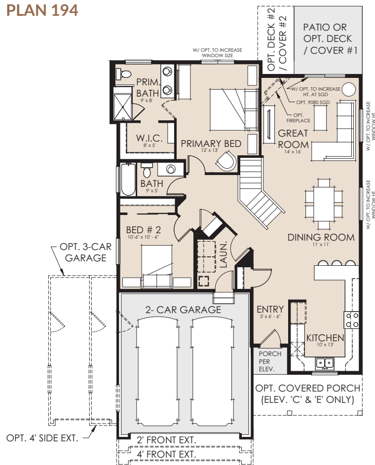
MAIN LEVEL 1,379 SF
