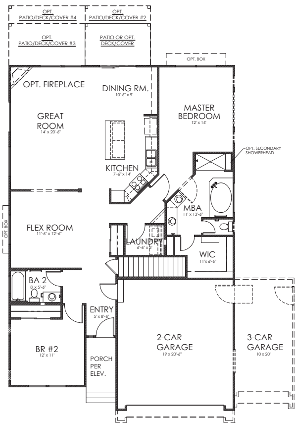
MAIN LEVEL 1,654 SF
