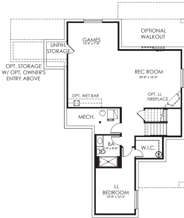
LOWER LEVEL OPTIONAL FINISH 1,016 SF
