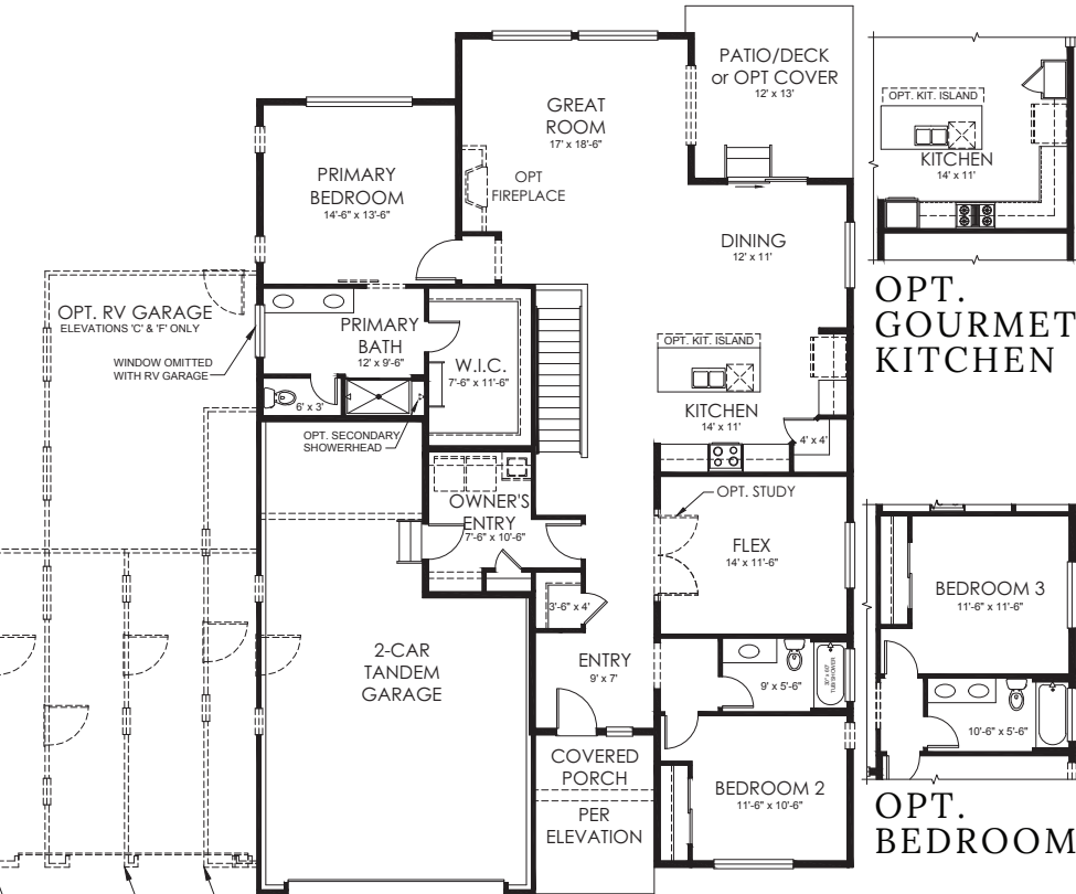
MAIN LEVEL 1,950 SF
