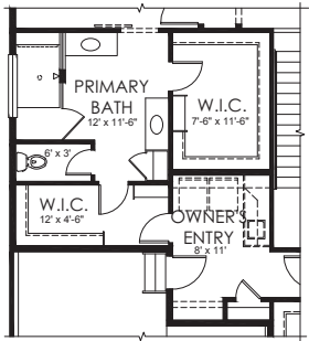
OPT. GRAND SUITE +92 SF
