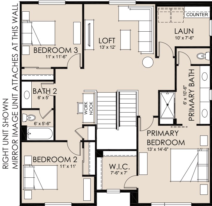
UPPER LEVEL 1,346 SF
