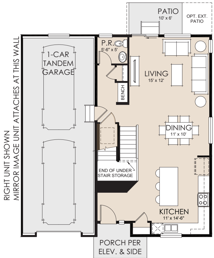
MAIN LEVEL 819 SF
