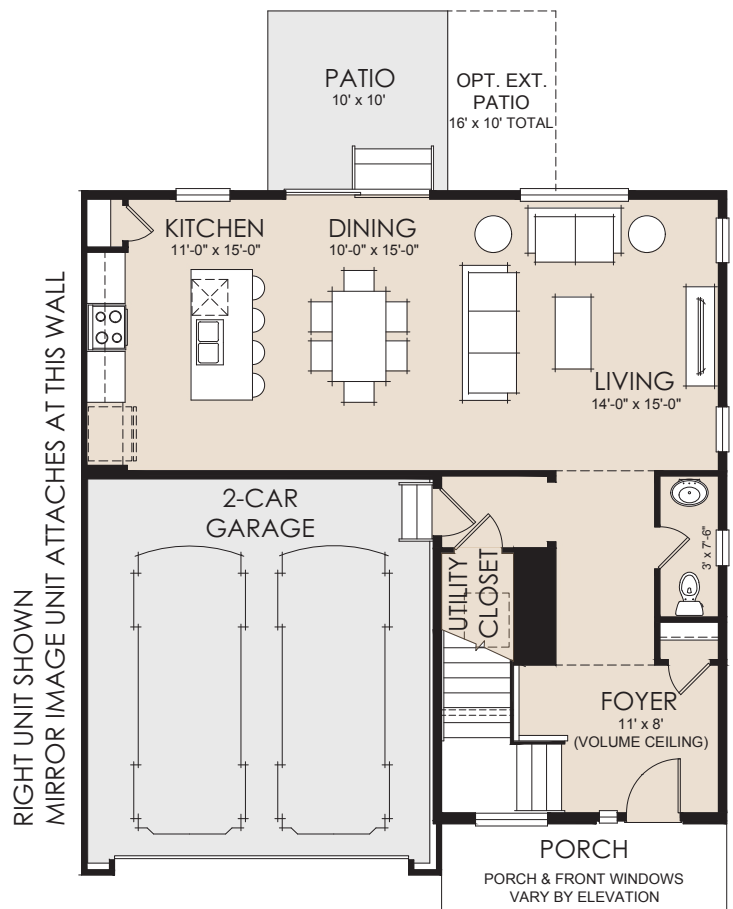
MAIN LEVEL 886 SF
