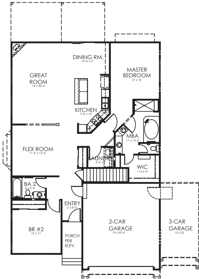
MAIN LEVEL 2096 SF
