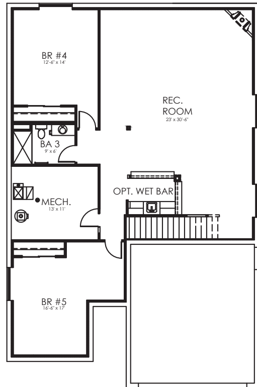
LOWER LEVEL OPTIONAL FINISH 1475 SF
