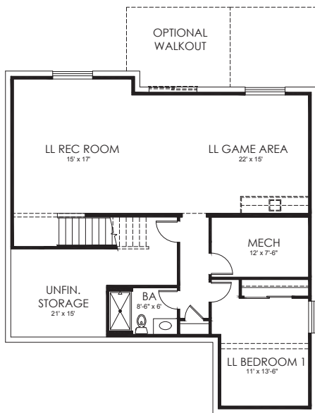
LOWER LEVEL OPTIONAL FINISH 964 SF
