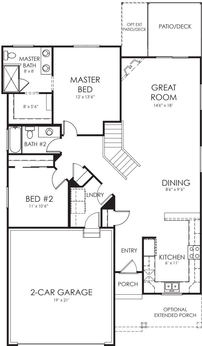
MAIN FLOOR 1,378 SF
