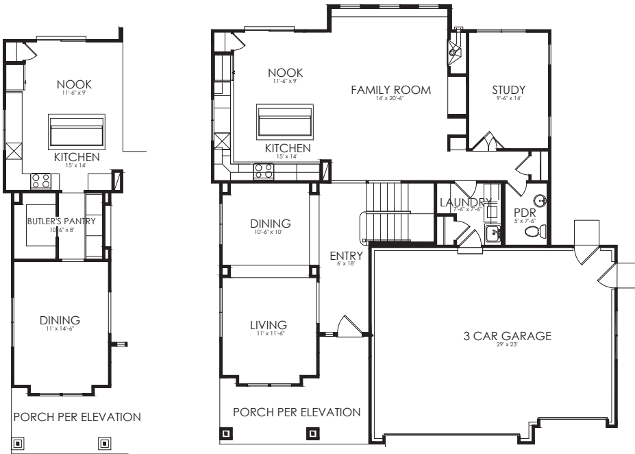
MAIN LEVEL 1,390 SF
